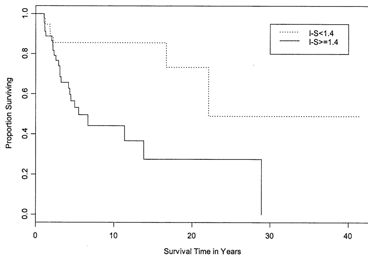
Figure 2. Survival* curve of fellow eyes from initial unilateral keratoconus (KC) diagnosis to the development of bilateral KC stratified by inferior-superior (I-S) dioptric asymmetry values. Top line, The survival curve of the fellow eyes with I-S<1.4; bottom line, the survival curve of the fellow eyes with I-S≥1.4. *Defined as the period during which the normal eyes remained normal.
