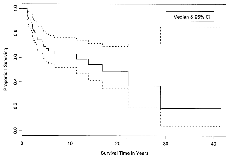
Figure 1. Survival* curve of all fellow eyes from initial unilateral keratoconus (KC) diagnosis to the development of bilateral KC. Top line, Upper 95% confidence intervals of the survival curve; middle line, survival curve of estimated developing time and proportions; bottom line, lower 95% confidence intervals of the survival curve. *Defined as the period during which the normal eyes remained normal.
