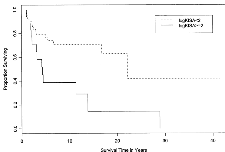
Figure 3. Survival curve of fellow eyes from initial unilateral keratoconus (KC) diagnosis to the development of bilateral KC stratified by keratoconus percentage (logKISA) values. Top line, The survival* curve of the fellow eyes with logKISA < 2; bottom line, the survival curve of the fellow eyes with logKISA ≥ 2. *Defined as the period during which the normal eyes remained normal.
